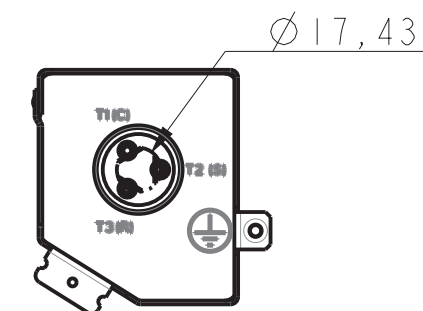
Schematic of Connection
